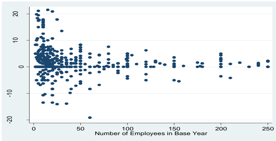
Fig. 1. Scatter Plot of Firm Size against Employment Growth
