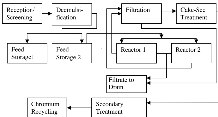
Fig. 1. Chromium Recovery Plant Flow Sheet.
